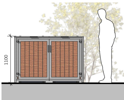
3 Bins Front Elevation 1 : 50
